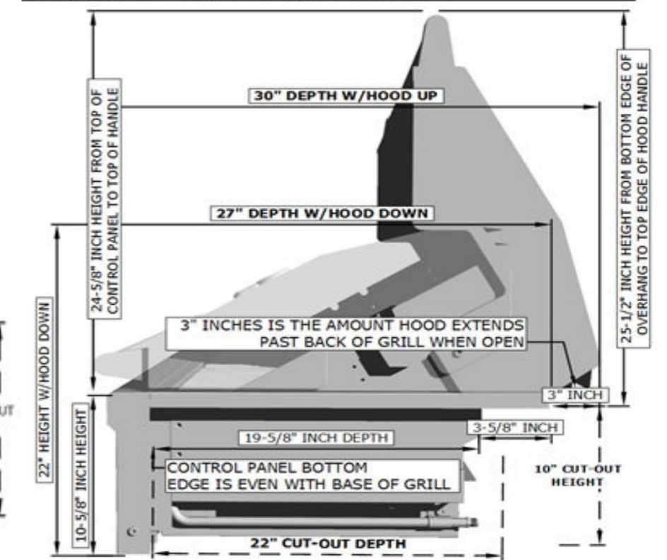
HOOD OPEN - RIGHT SIDE VIEW
